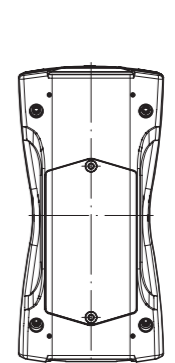
Base - external view
