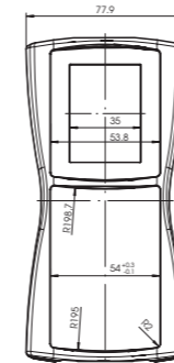
Lid - external view
